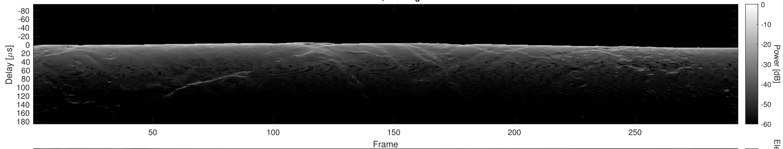
Orbit 18970, Cluttergram
