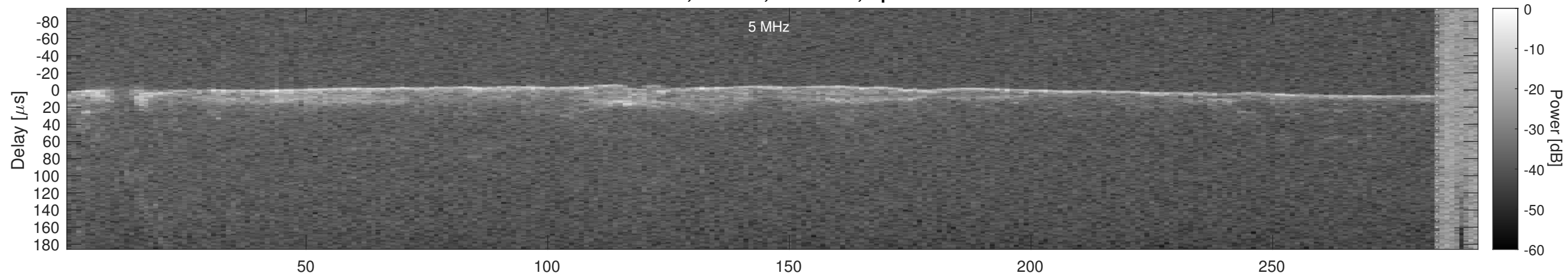
Orbit 18970, Cluttergram
