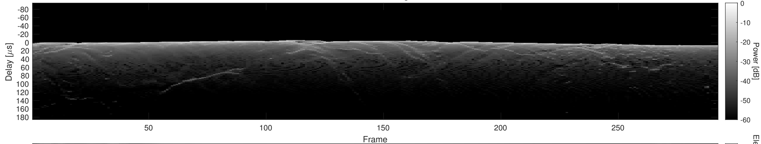
Orbit 18970, Cluttergram
