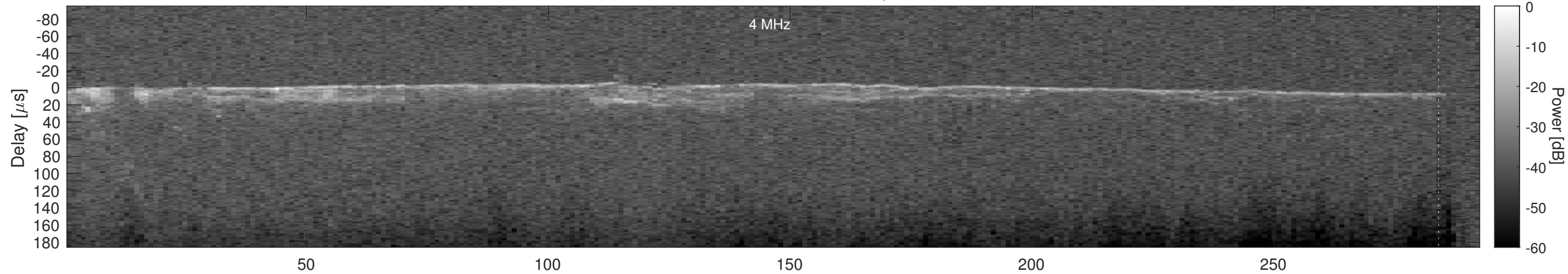
Orbit 18970, Cluttergram
