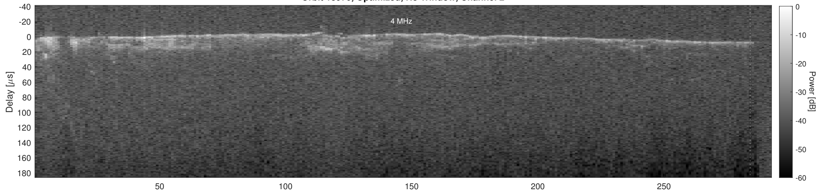
Orbit 18970, Cluttergram
