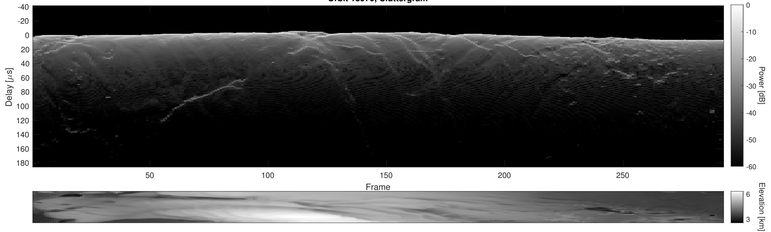
Orbit 18970, Cluttergram
