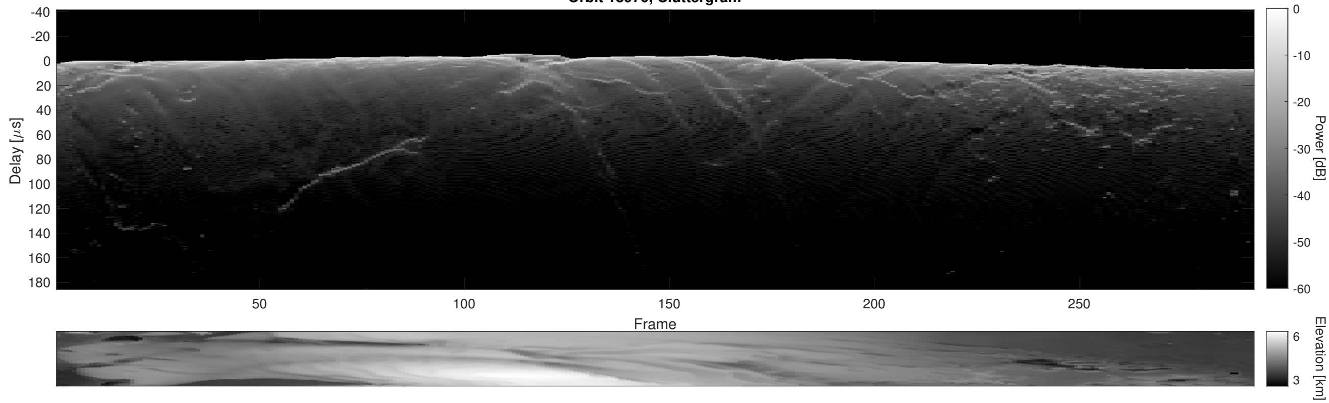
Orbit 18970, Cluttergram
