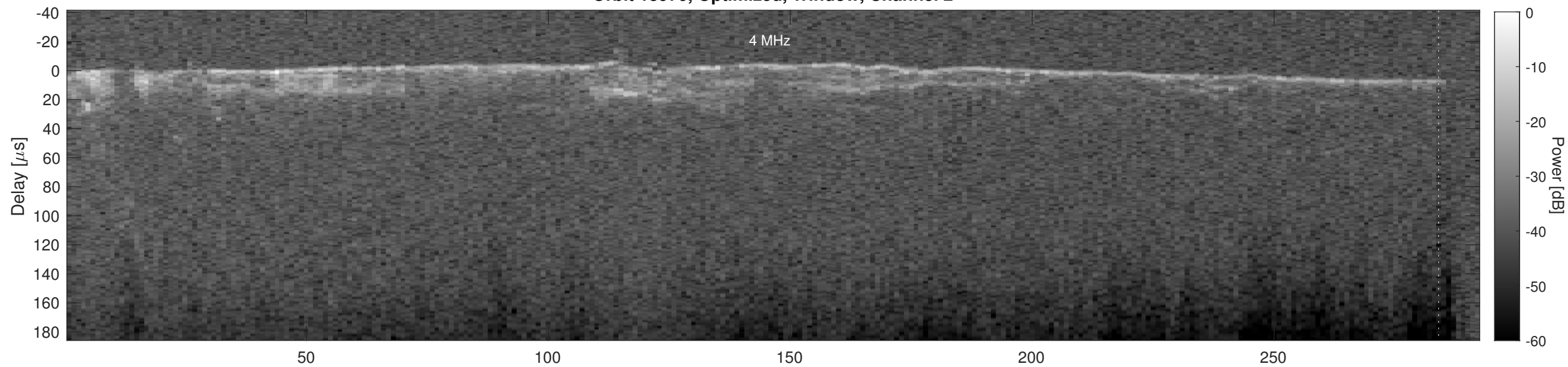
Orbit 18970, Cluttergram
