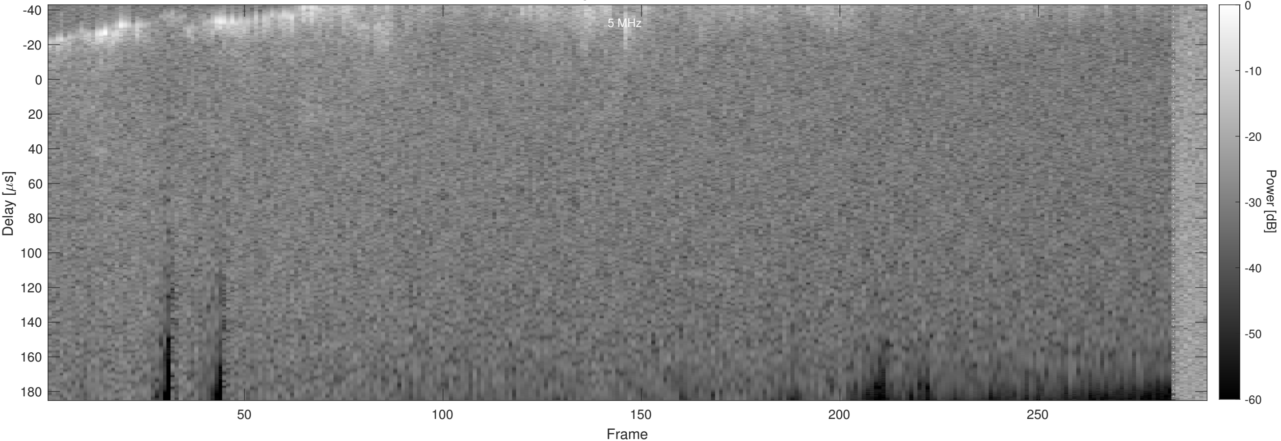
Orbit 18971, Chapman, No Window, Channel 2
