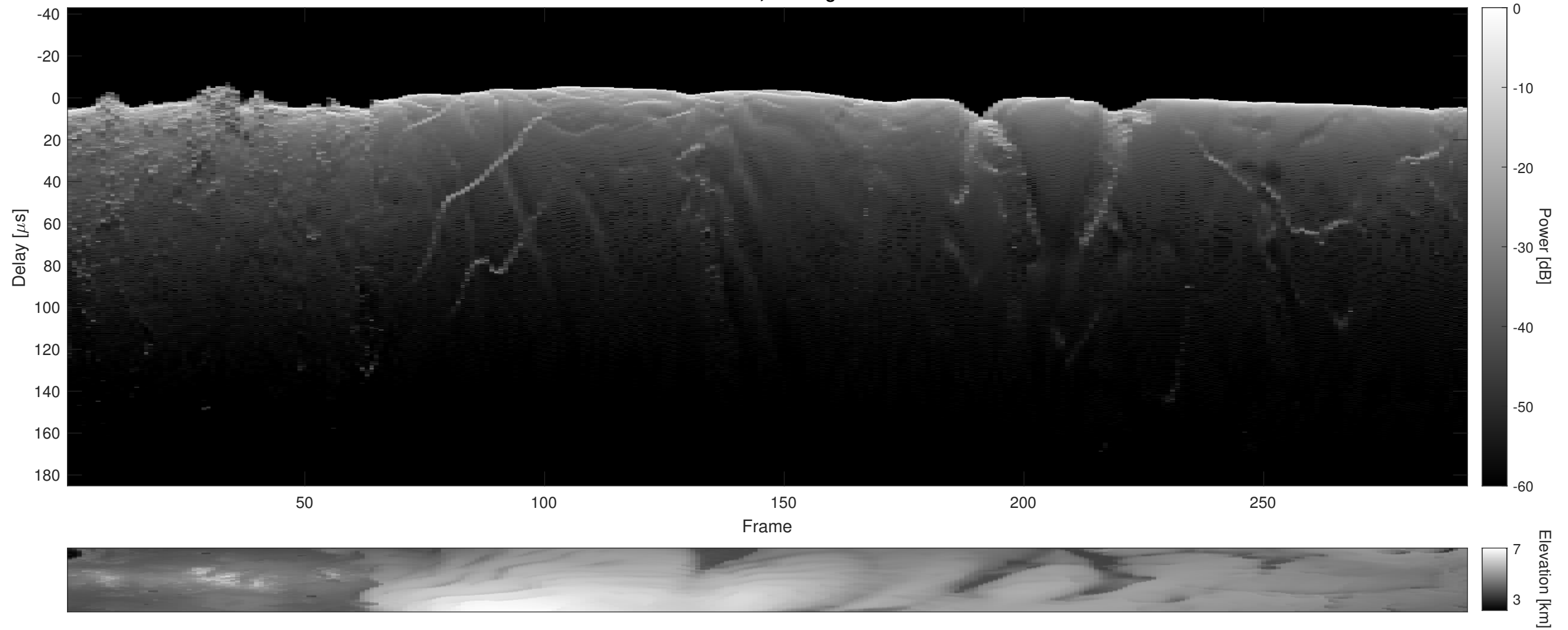
Orbit 18971, Cluttergram
