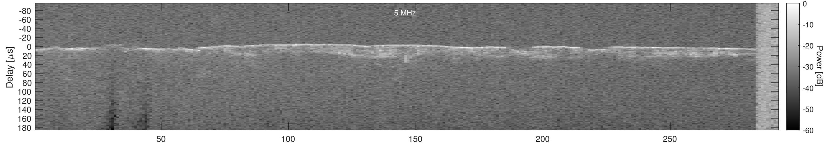
Orbit 18971, Cluttergram
