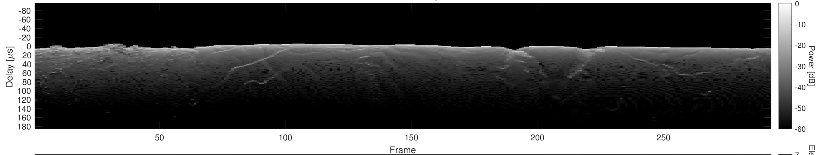
Orbit 18971, Cluttergram
