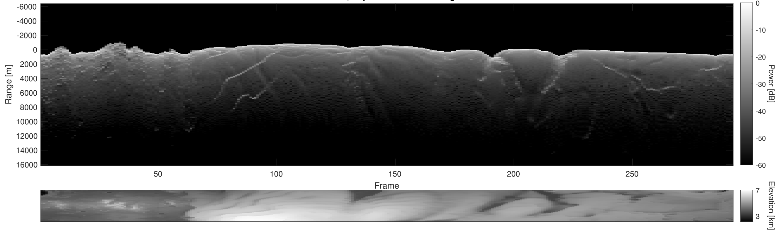
Orbit 18971, Depth-Corrected Cluttergram
