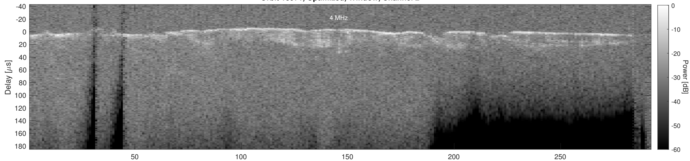
Orbit 18971, Cluttergram
