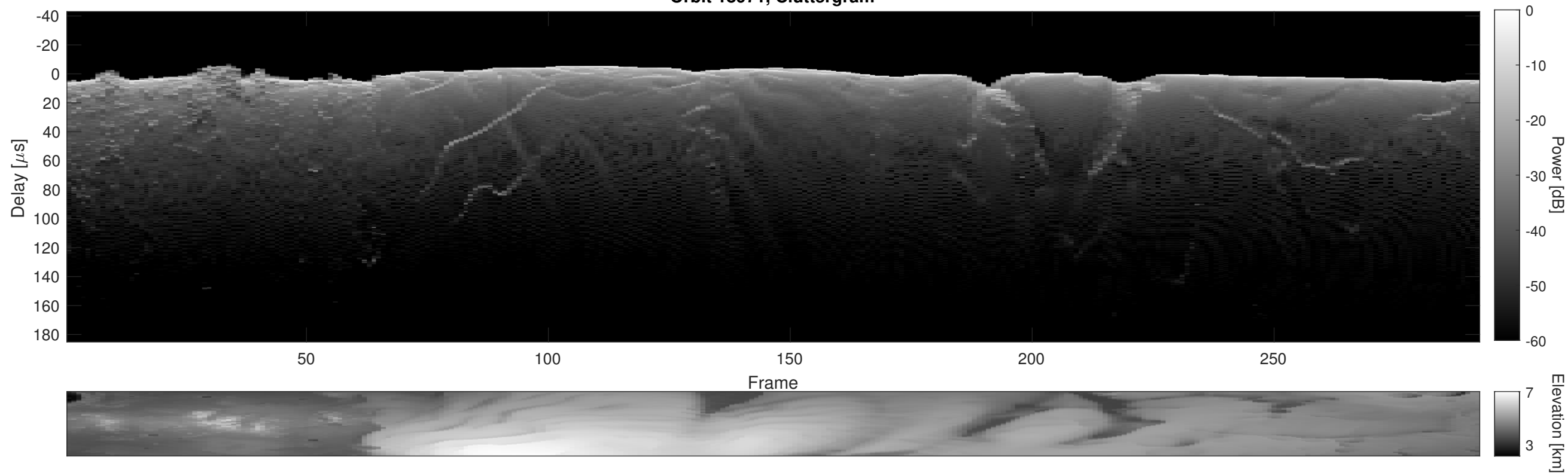
Orbit 18971, Cluttergram
