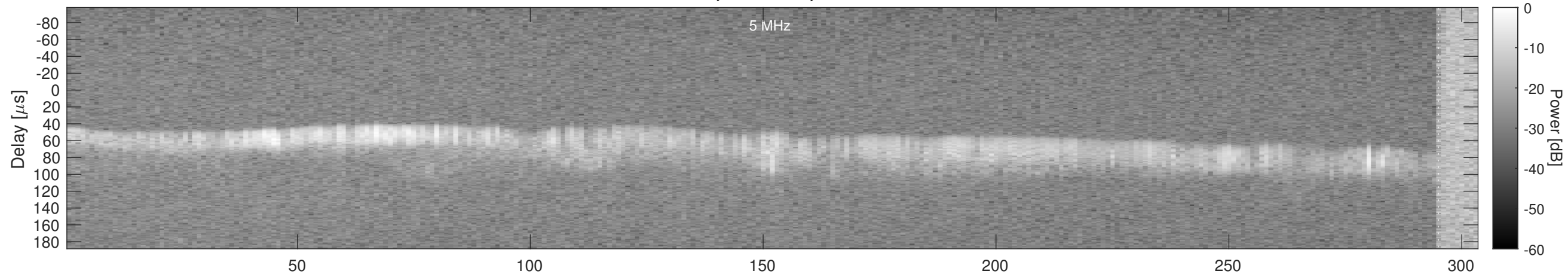
Orbit 18974, Window, Channel 1, Chapman
