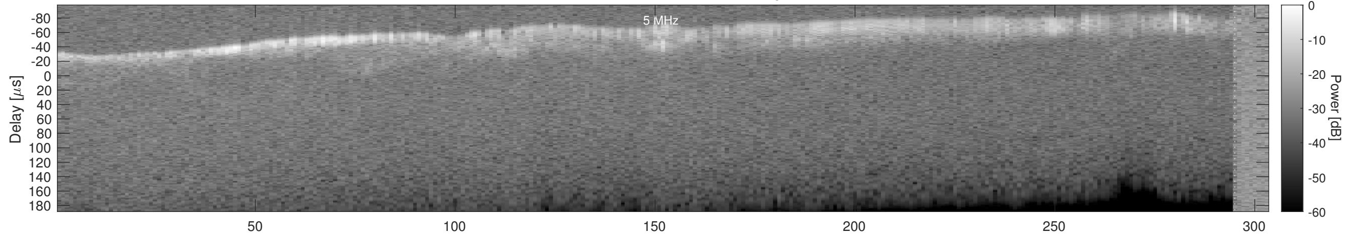
Orbit 18974, Window, Channel 1, Optimized
