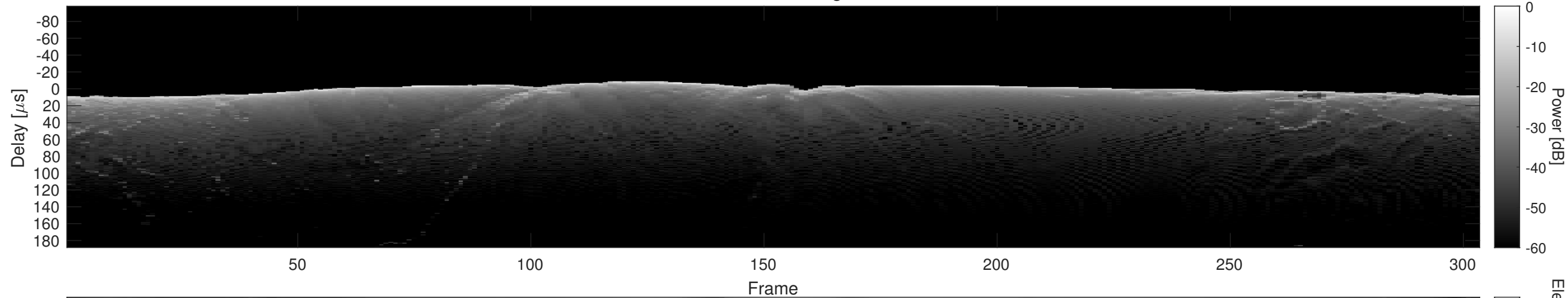
Orbit 18974, Cluttergram
