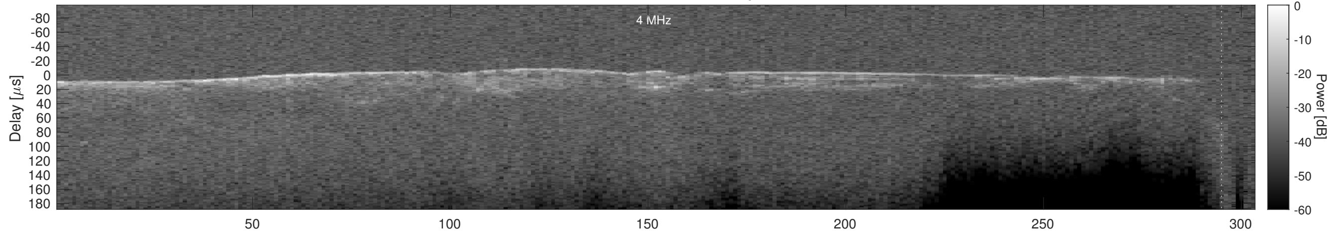
Orbit 18974, Cluttergram
