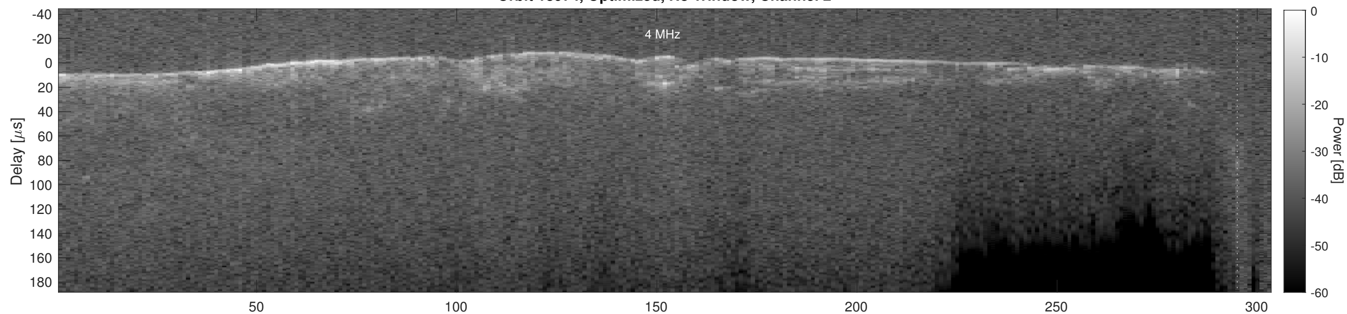
Orbit 18974, Cluttergram
