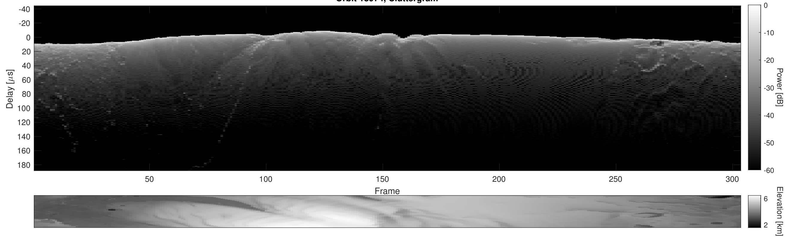
Orbit 18974, Cluttergram
