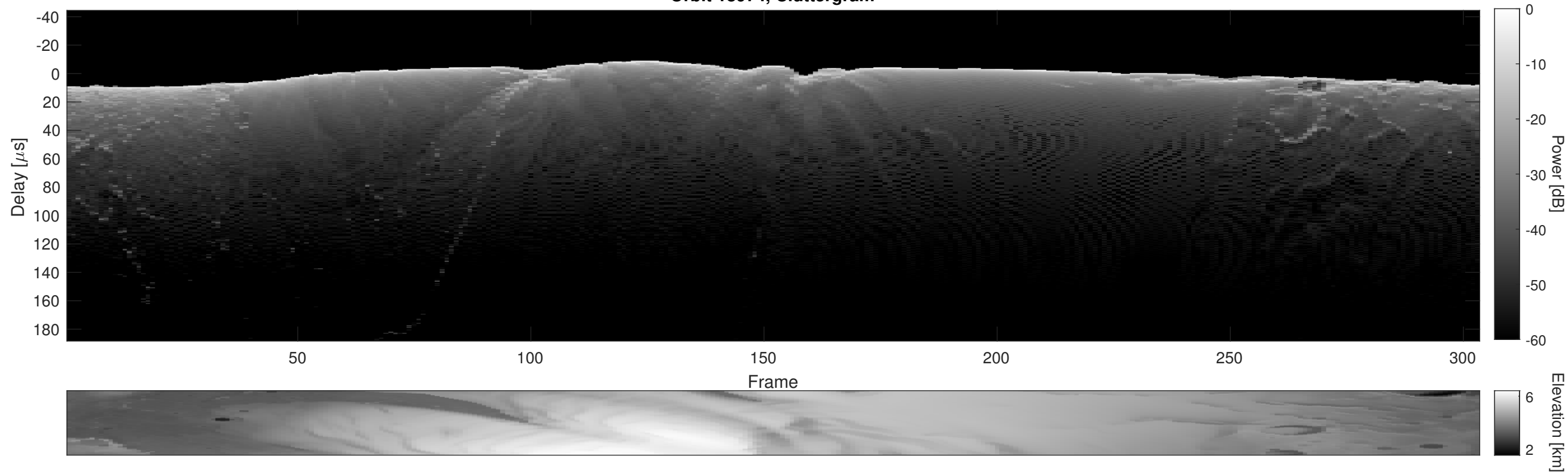
Orbit 18974, Cluttergram
