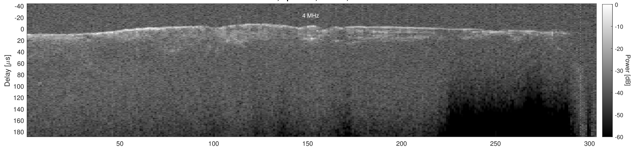
Orbit 18974, Cluttergram
