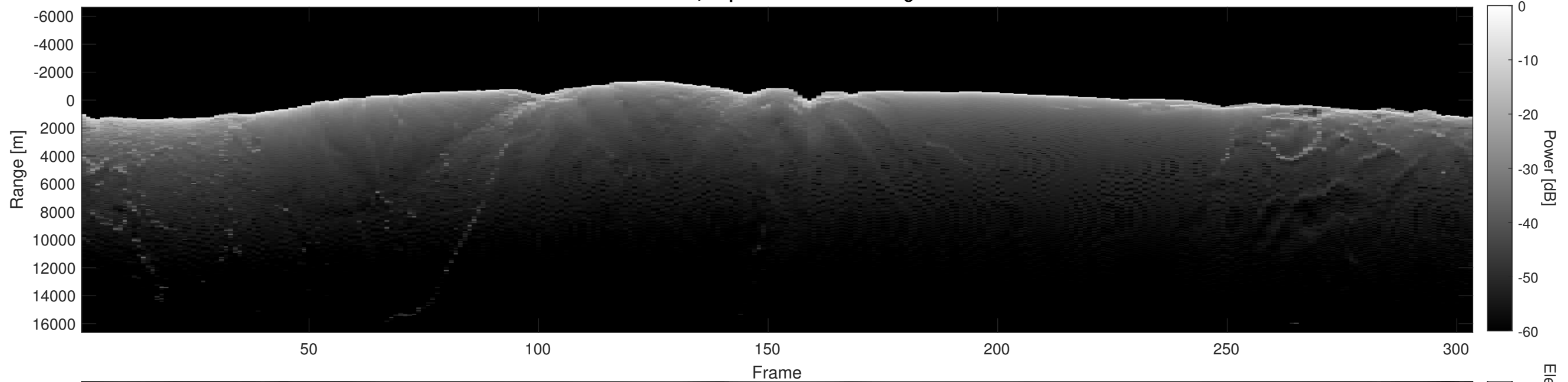
Orbit 18974, Depth-Corrected Cluttergram
