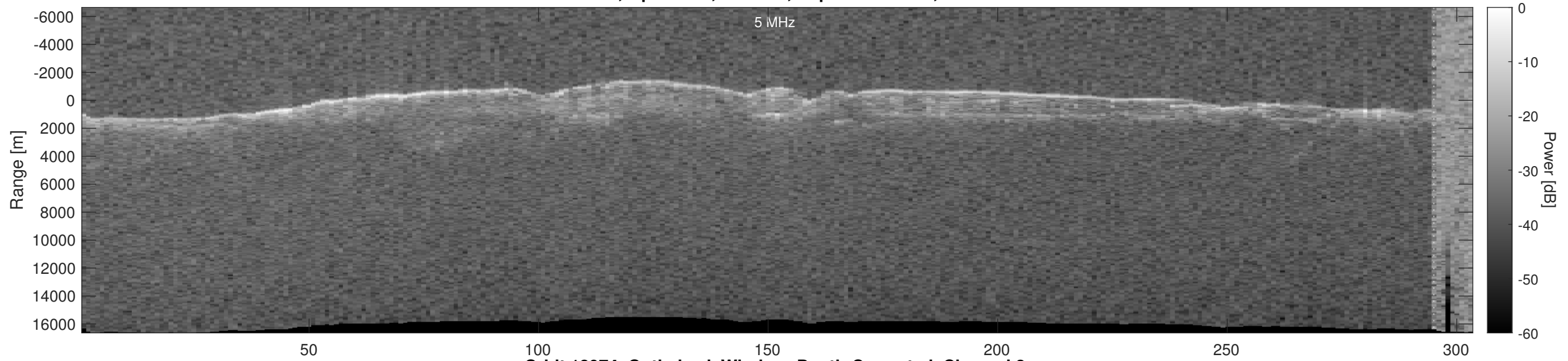
Orbit 18974, Optimized, Window, Depth-Corrected, Channel 2
