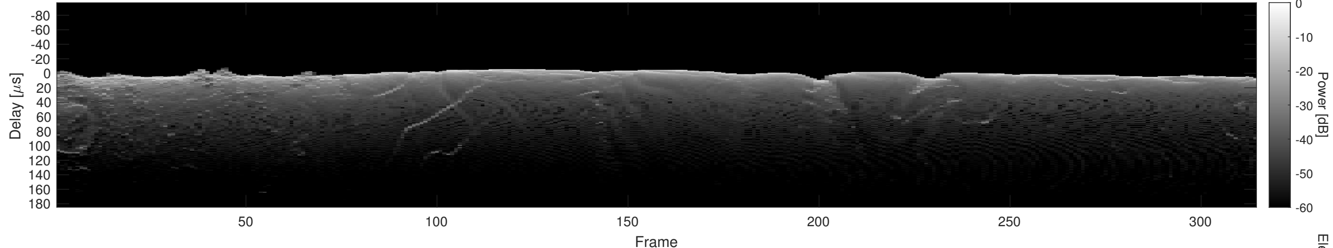
Orbit 18978, Cluttergram
