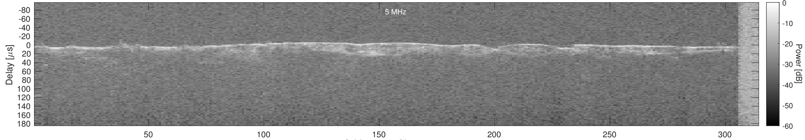
Orbit 18978, Cluttergram
