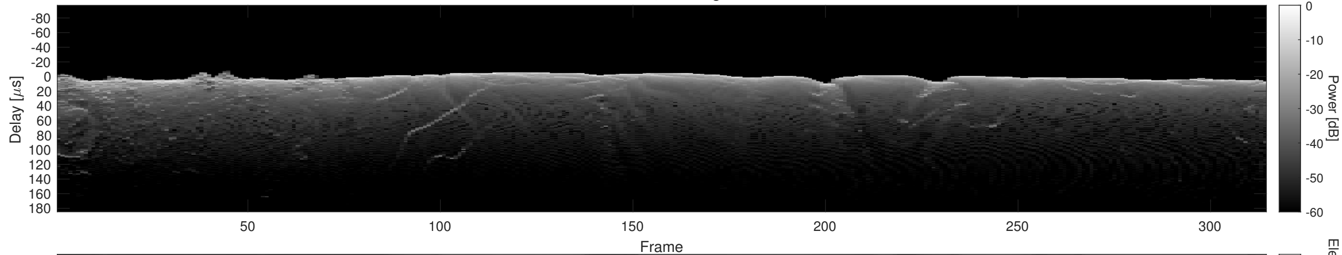
Orbit 18978, Cluttergram
