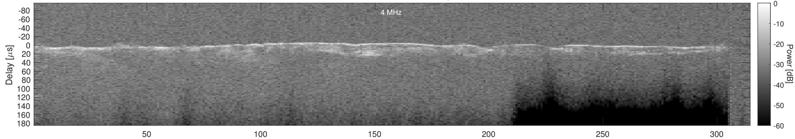
Orbit 18978, Cluttergram
