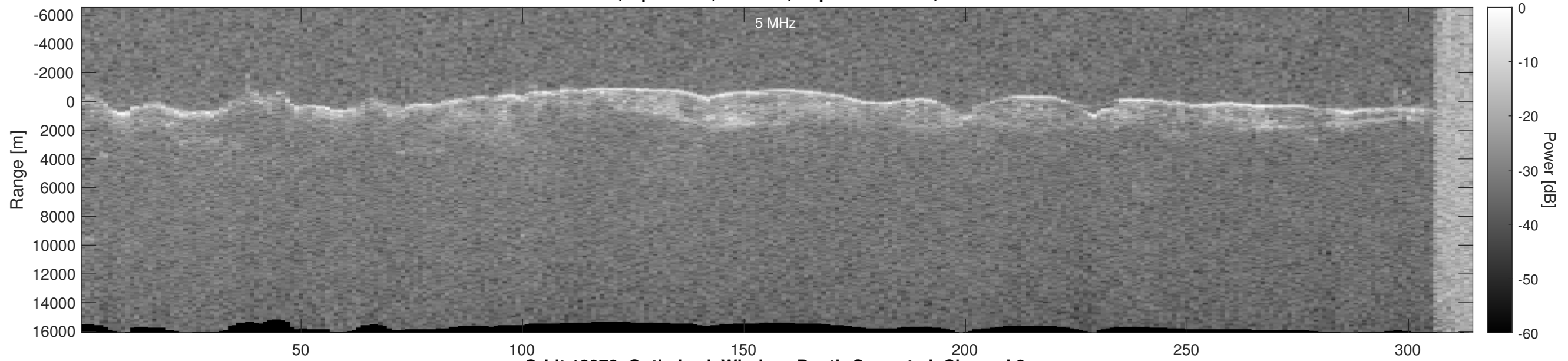
Orbit 18978, Optimized, Window, Depth-Corrected, Channel 2
