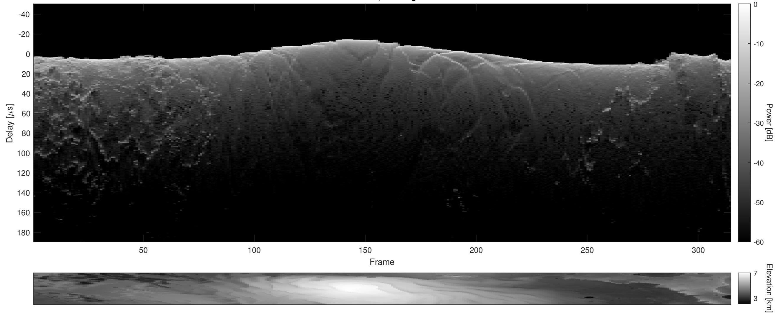
Orbit 18979, Cluttergram
