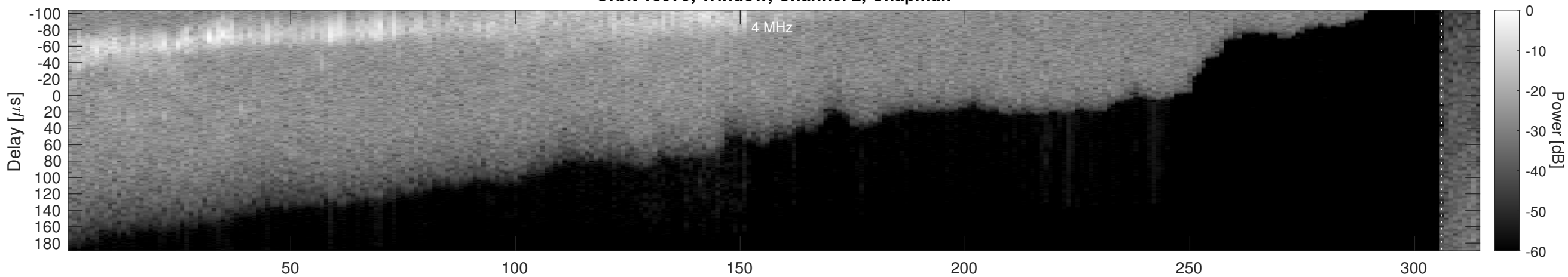
Orbit 18979, Window, Channel 2, Optimized
