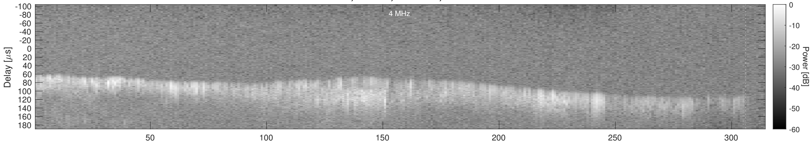
Orbit 18979, Window, Channel 2, Chapman
