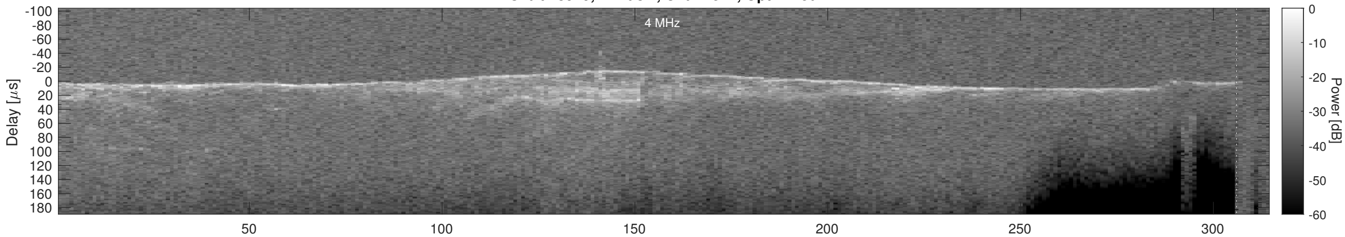
Orbit 18979, Cluttergram
