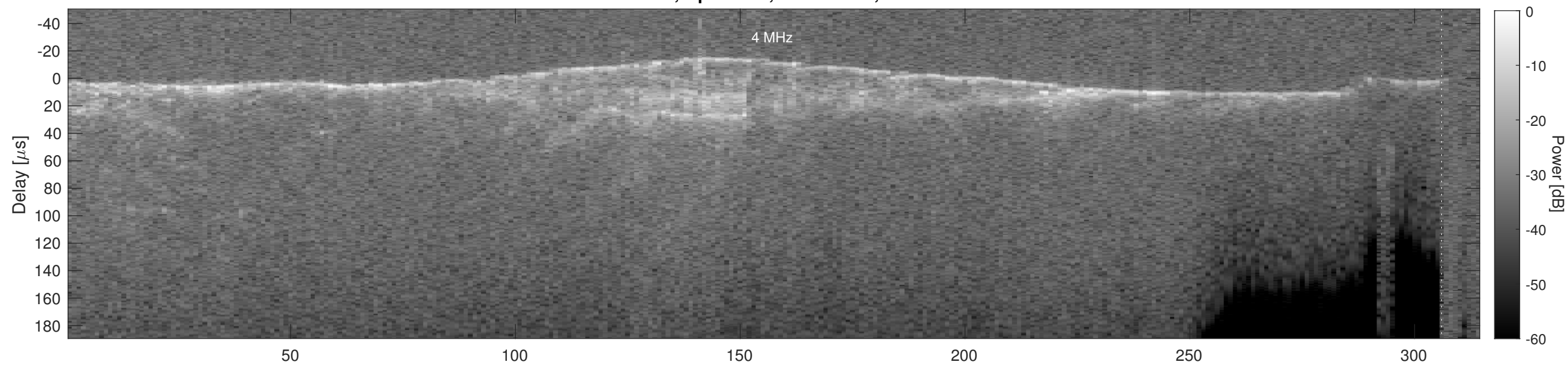
Orbit 18979, Cluttergram
