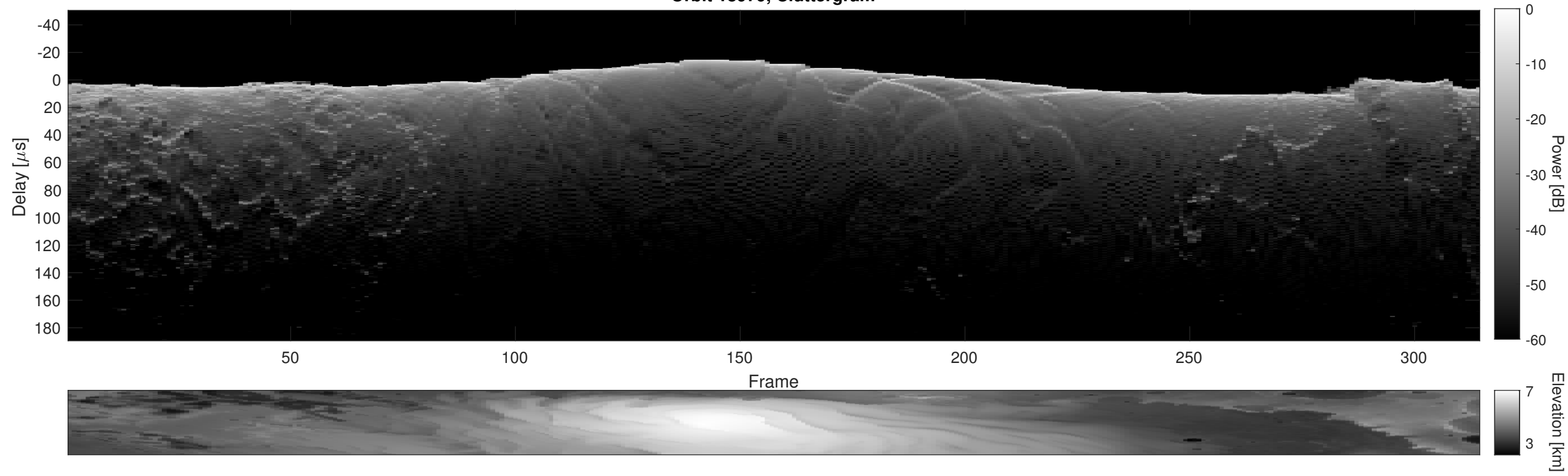
Orbit 18979, Cluttergram
