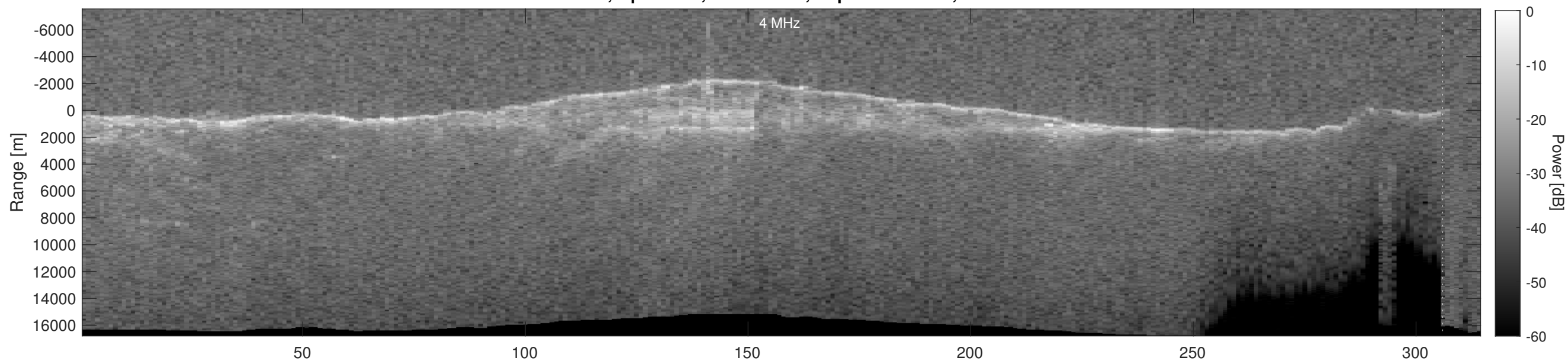
Orbit 18979, Depth-Corrected Cluttergram
