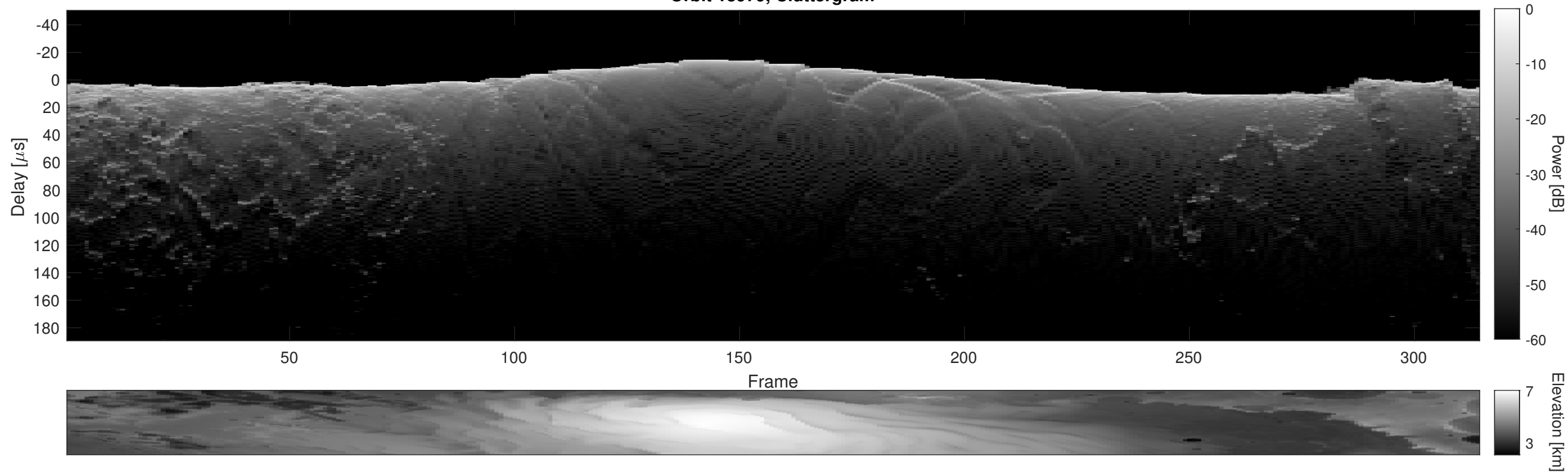
Orbit 18979, Cluttergram
