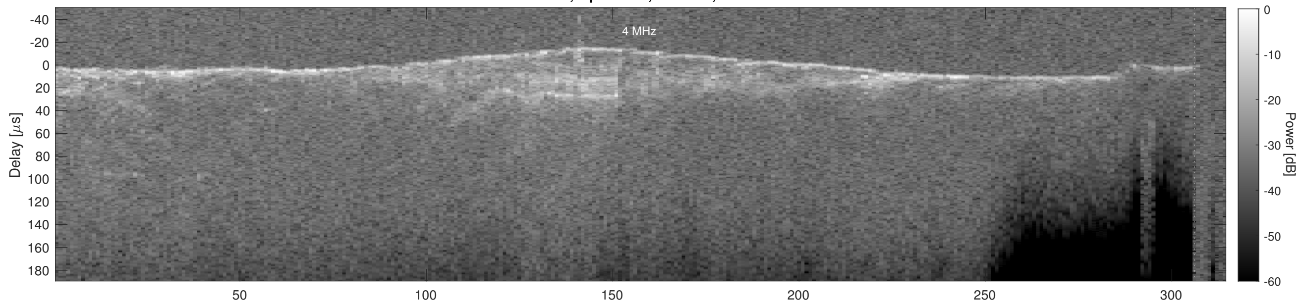
Orbit 18979, Cluttergram
