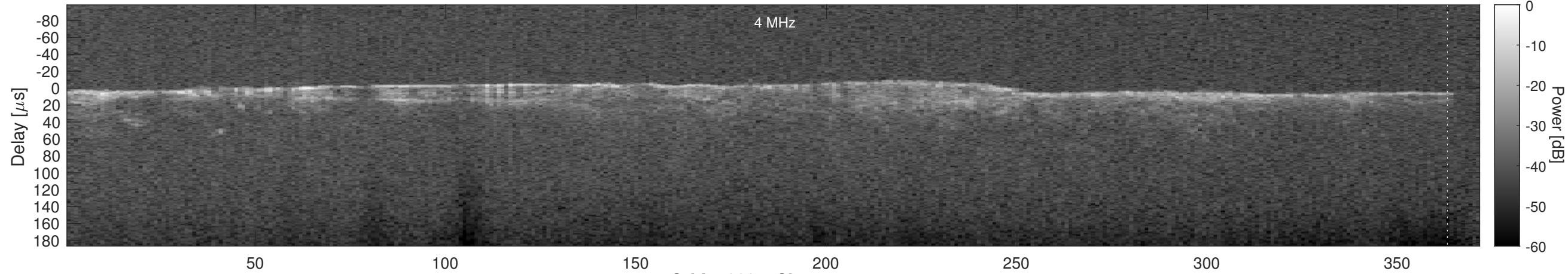
Orbit 19001, Cluttergram
