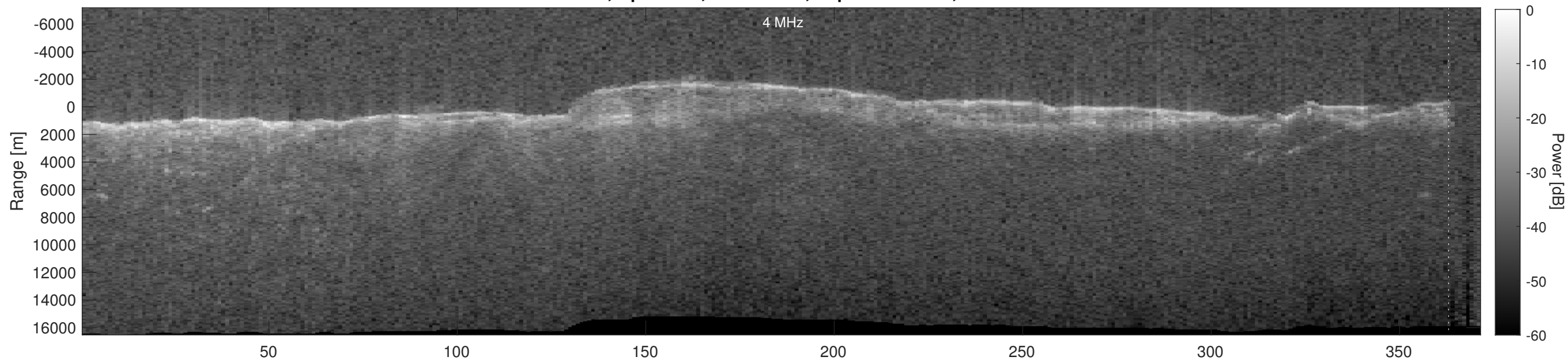
Orbit 19003, Depth-Corrected Cluttergram
