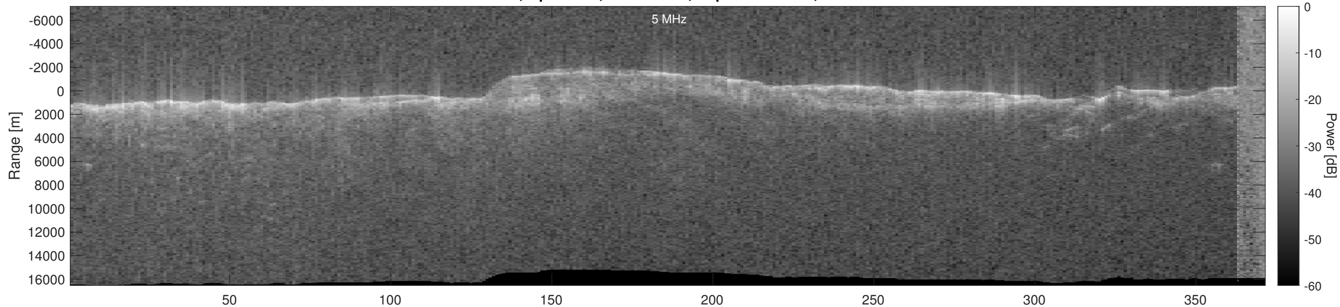
Orbit 19003, Optimized, No Window, Depth-Corrected, Channel 2
