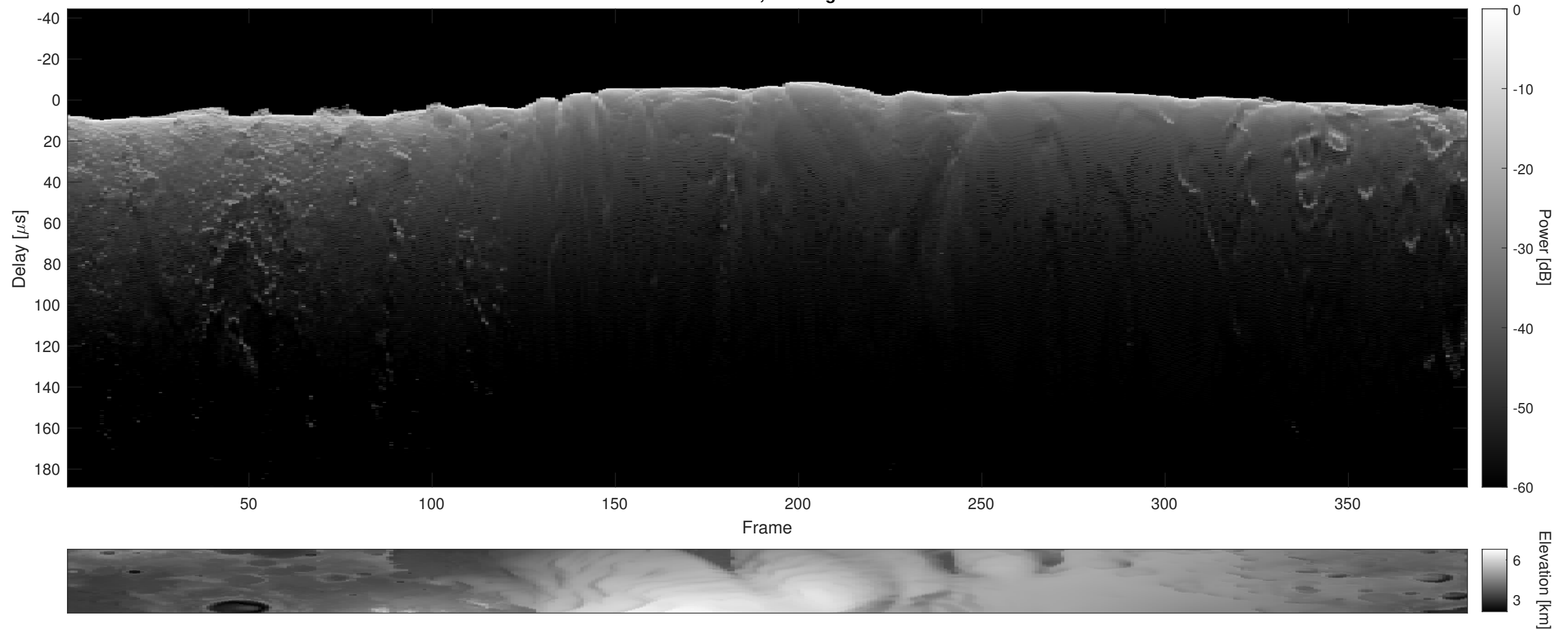
Orbit 19006, Cluttergram
