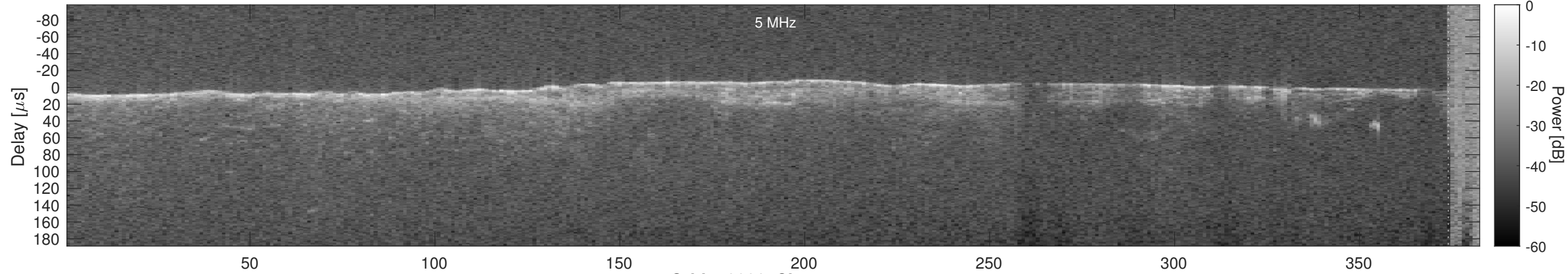
Orbit 19006, Cluttergram
