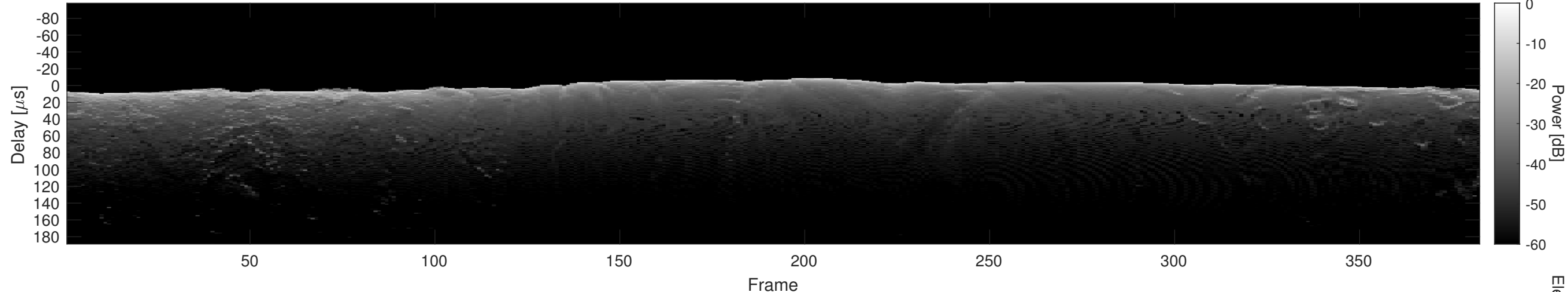
Orbit 19006, Cluttergram
