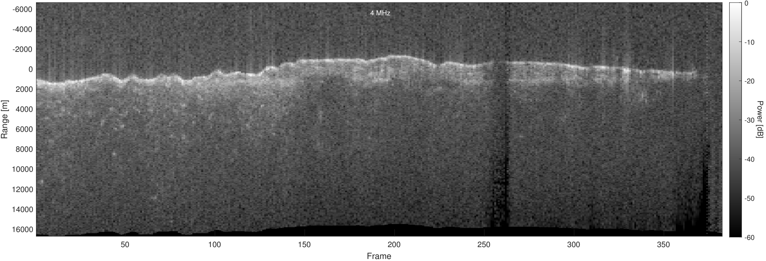
Orbit 19006, Optimized, No Window, Depth-Corrected, Channel 2
