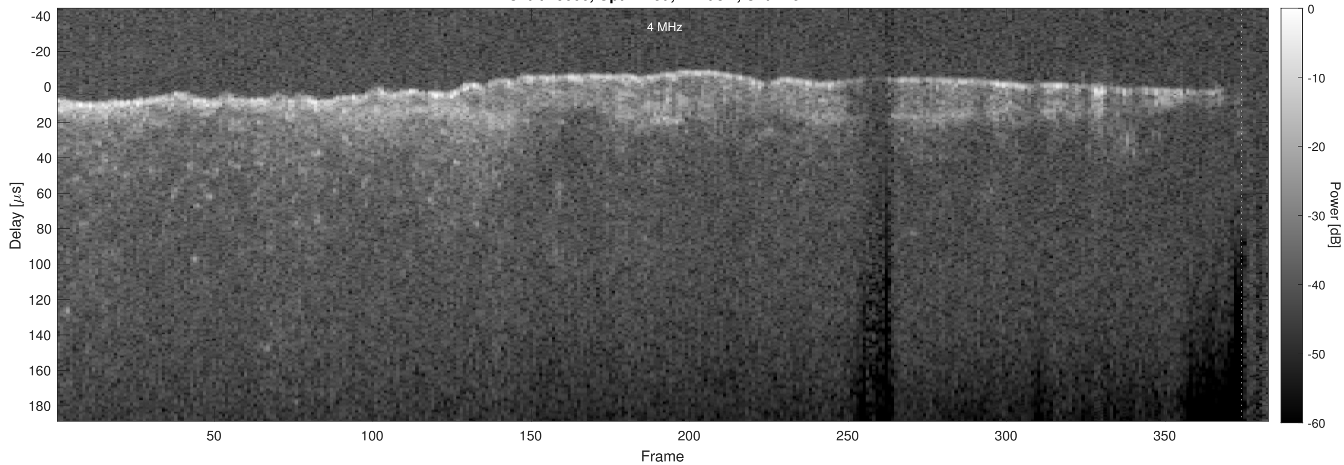
Orbit 19006, Optimized, Window, Channel 2
