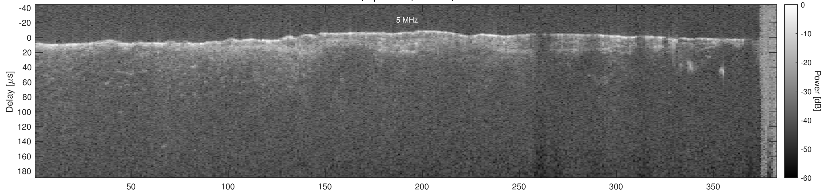
Orbit 19006, Optimized, Window, Channel 2
