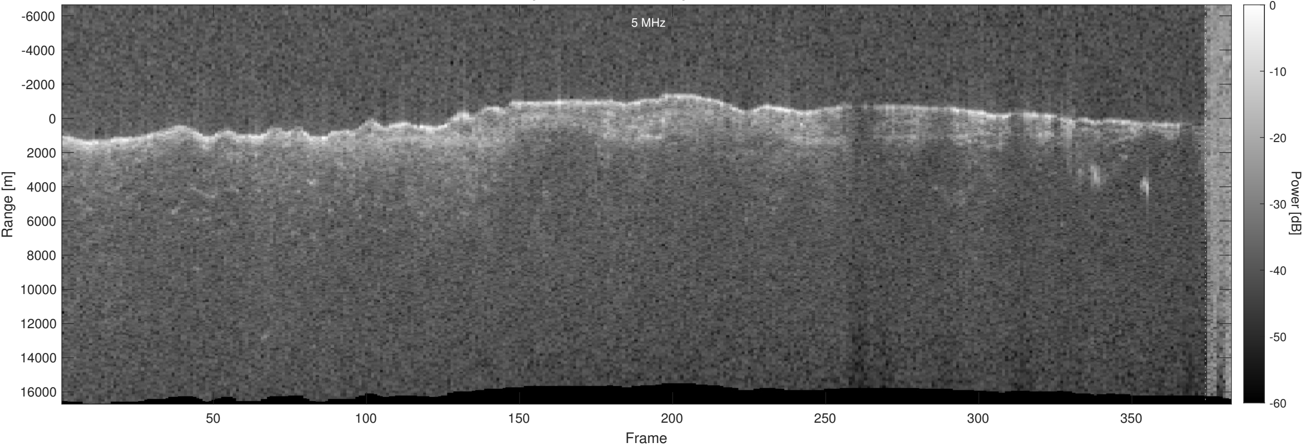
Orbit 19006, Optimized, Window, Depth-Corrected, Channel 2
