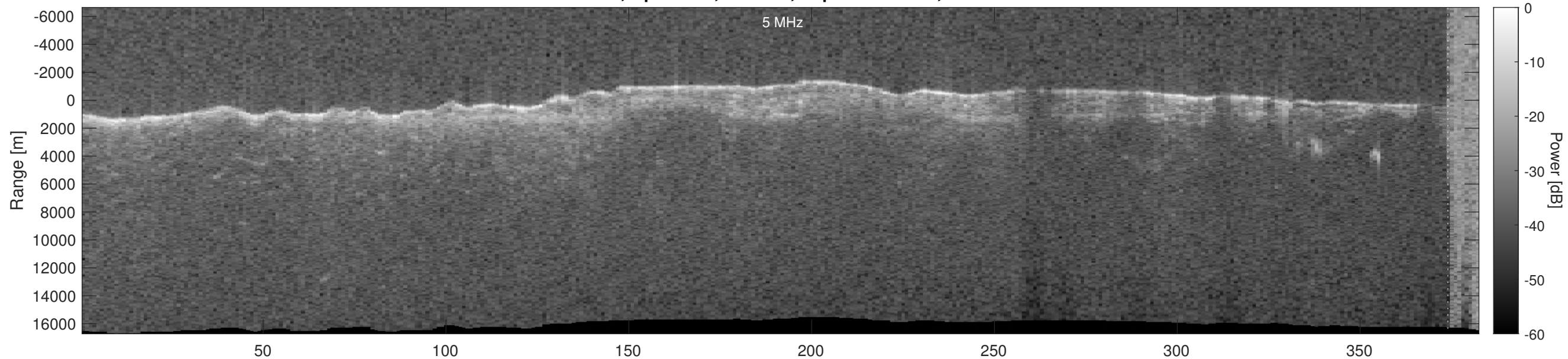
Orbit 19006, Optimized, Window, Depth-Corrected, Channel 2
