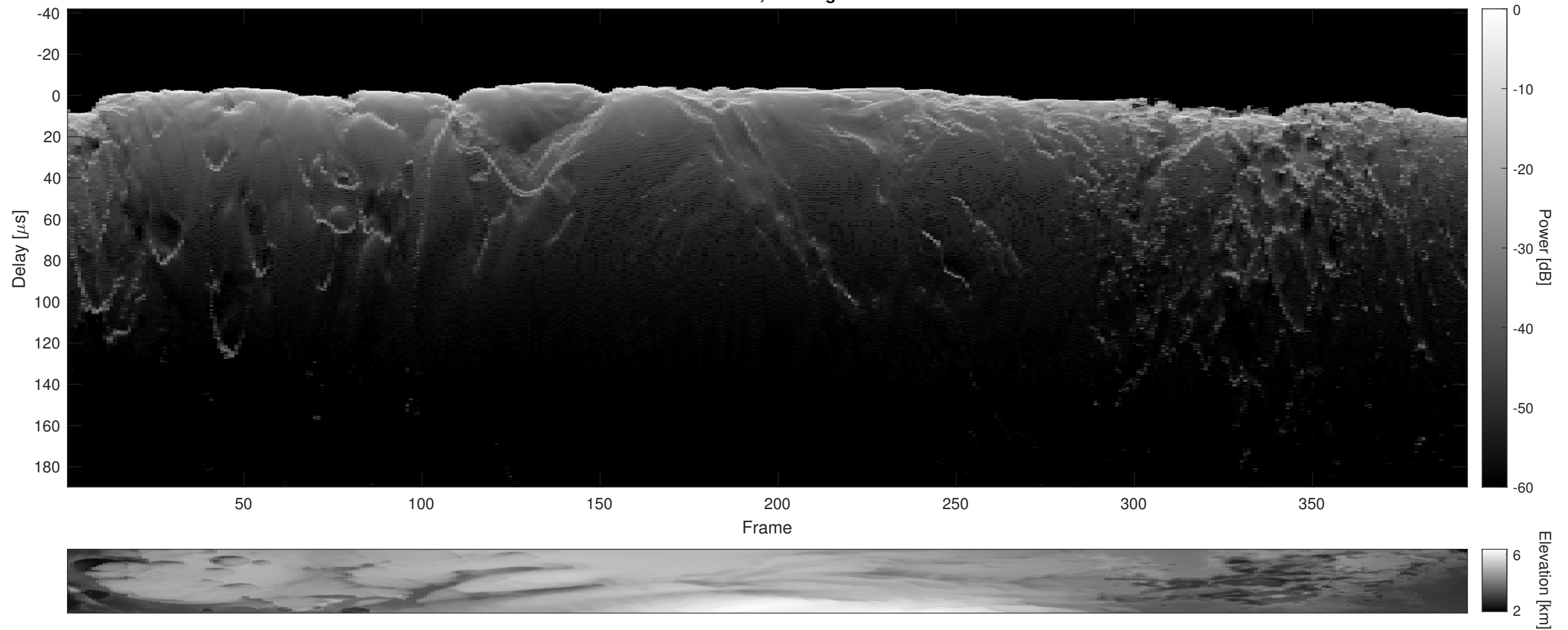
Orbit 19012, Cluttergram
