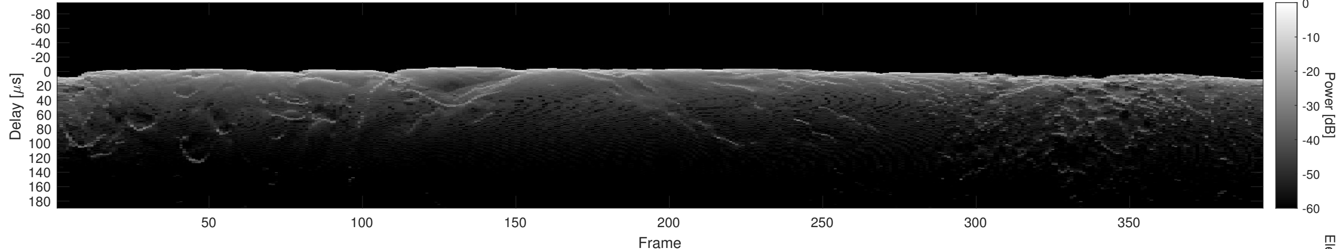
Orbit 19012, Cluttergram
