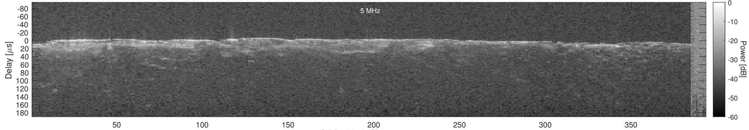
Orbit 19012, Cluttergram
