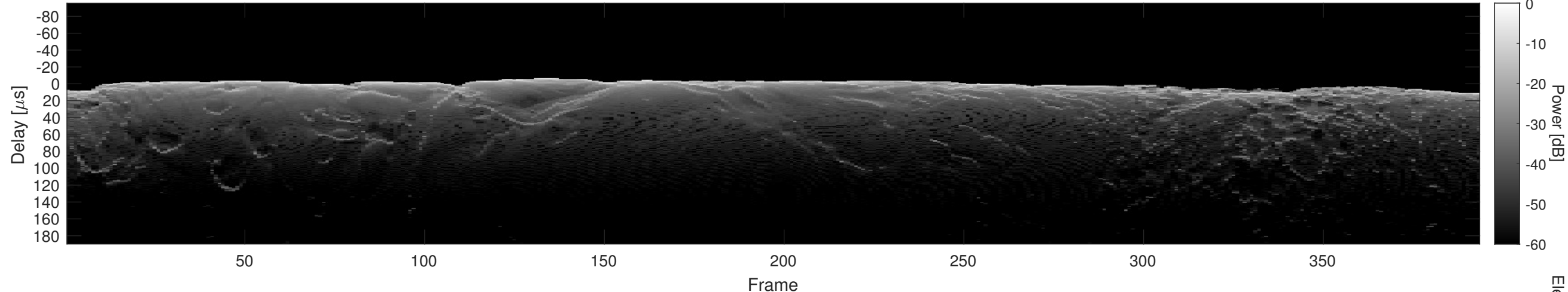
Orbit 19012, Cluttergram
