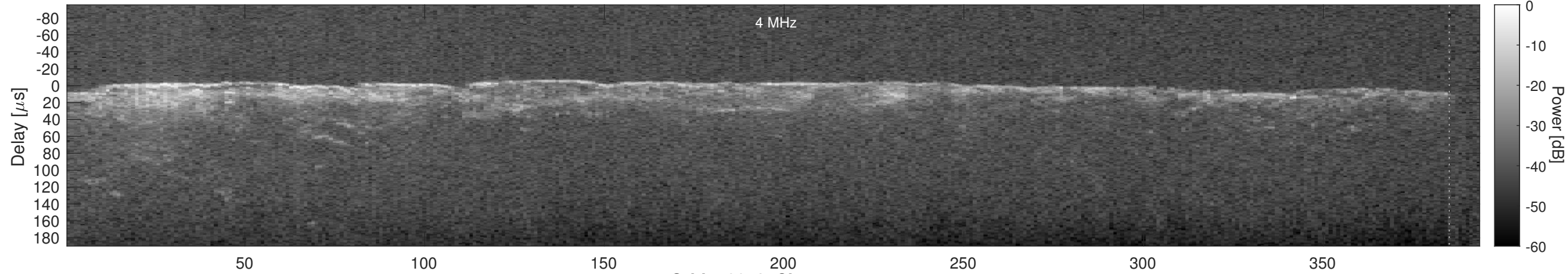
Orbit 19012, Cluttergram
