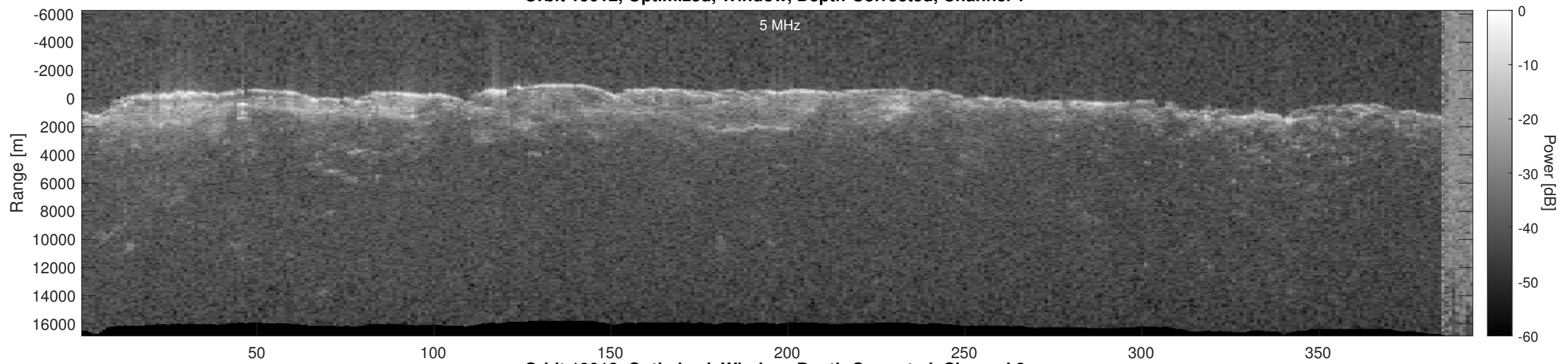
Orbit 19012, Optimized, Window, Depth-Corrected, Channel 2
