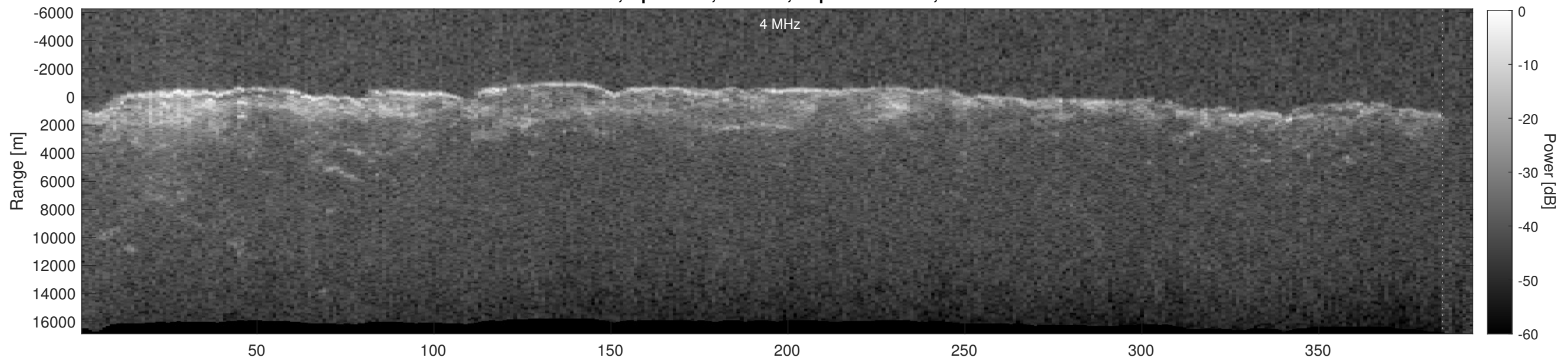
Orbit 19012, Depth-Corrected Cluttergram
