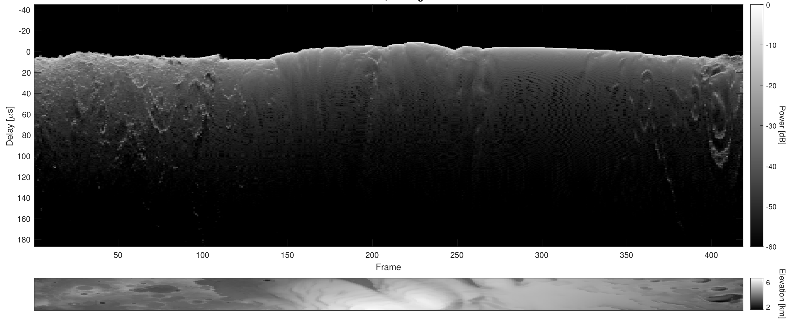
Orbit 19020, Cluttergram
