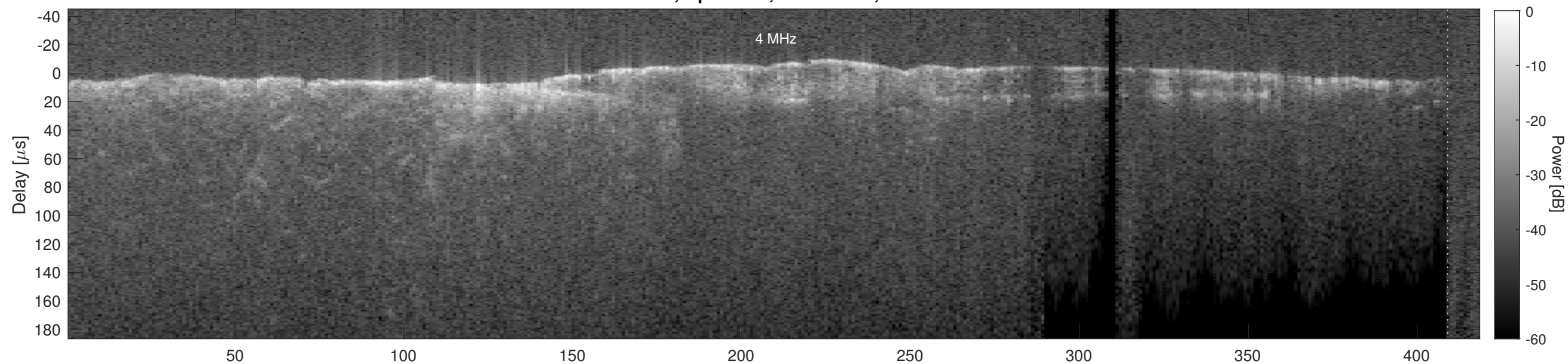
Orbit 19020, Cluttergram
