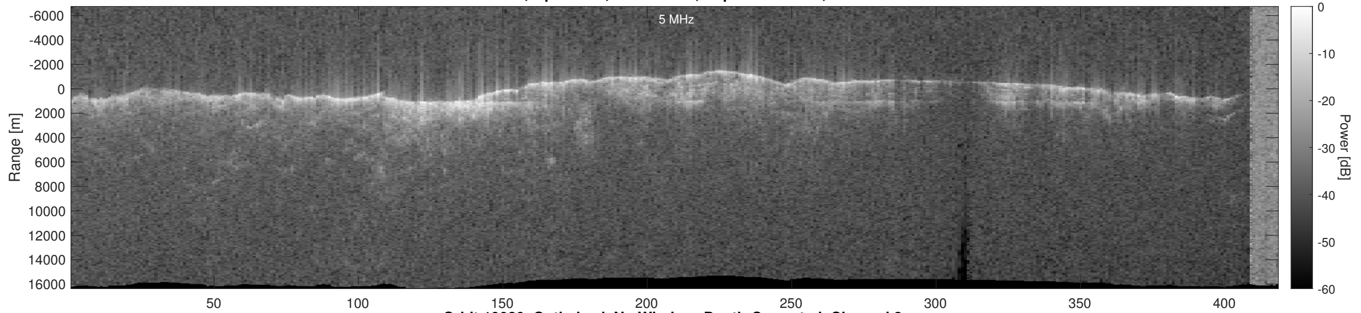
Orbit 19020, Optimized, No Window, Depth-Corrected, Channel 2
