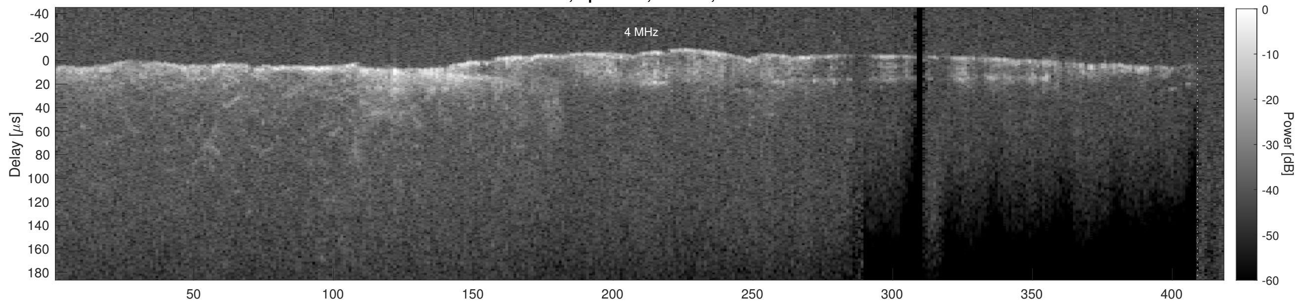
Orbit 19020, Cluttergram
