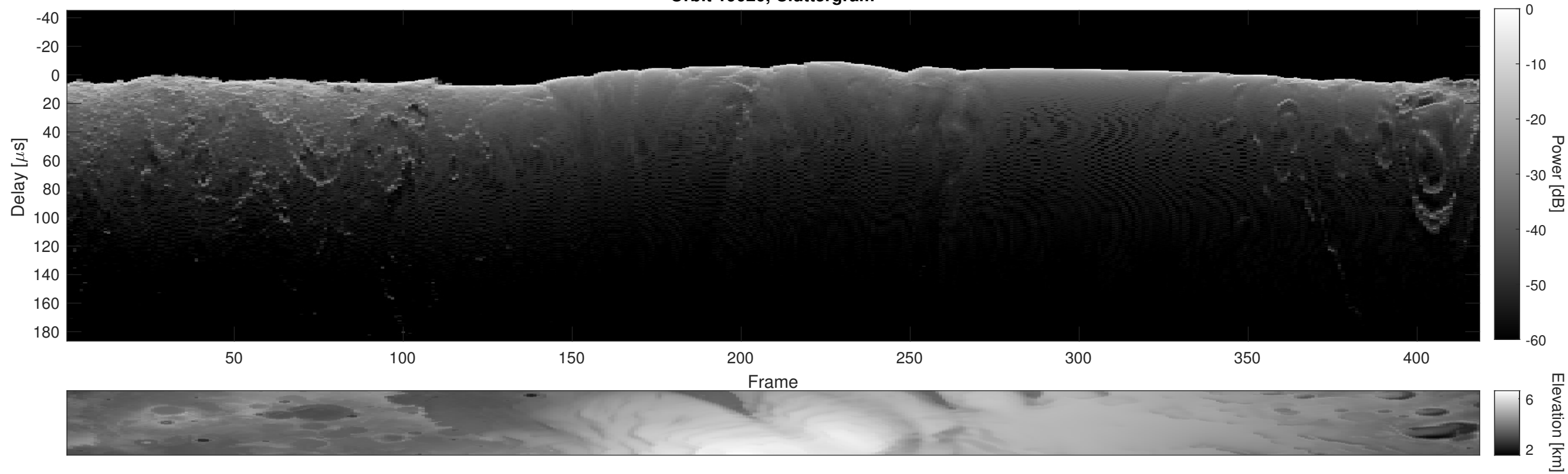
Orbit 19020, Cluttergram
