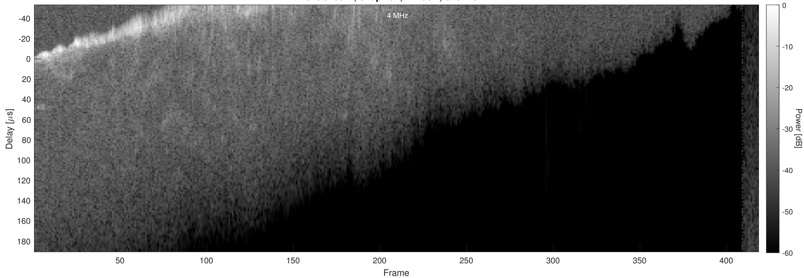
Orbit 19021, Chapman, Window, Channel 2
