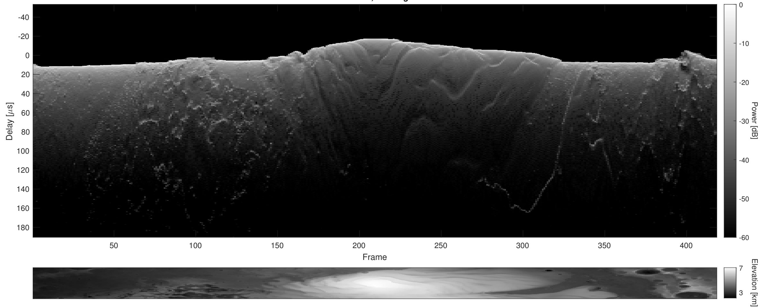
Orbit 19021, Cluttergram
