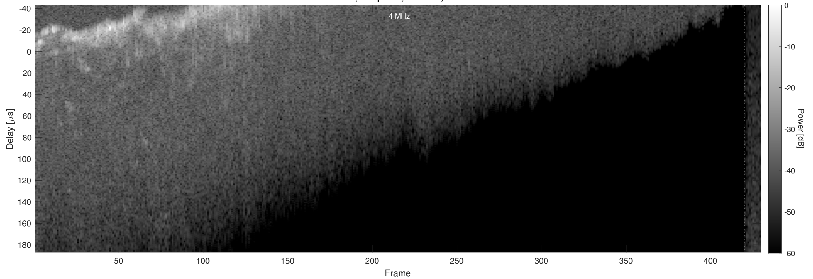
Orbit 19023, Chapman, Window, Channel 2
