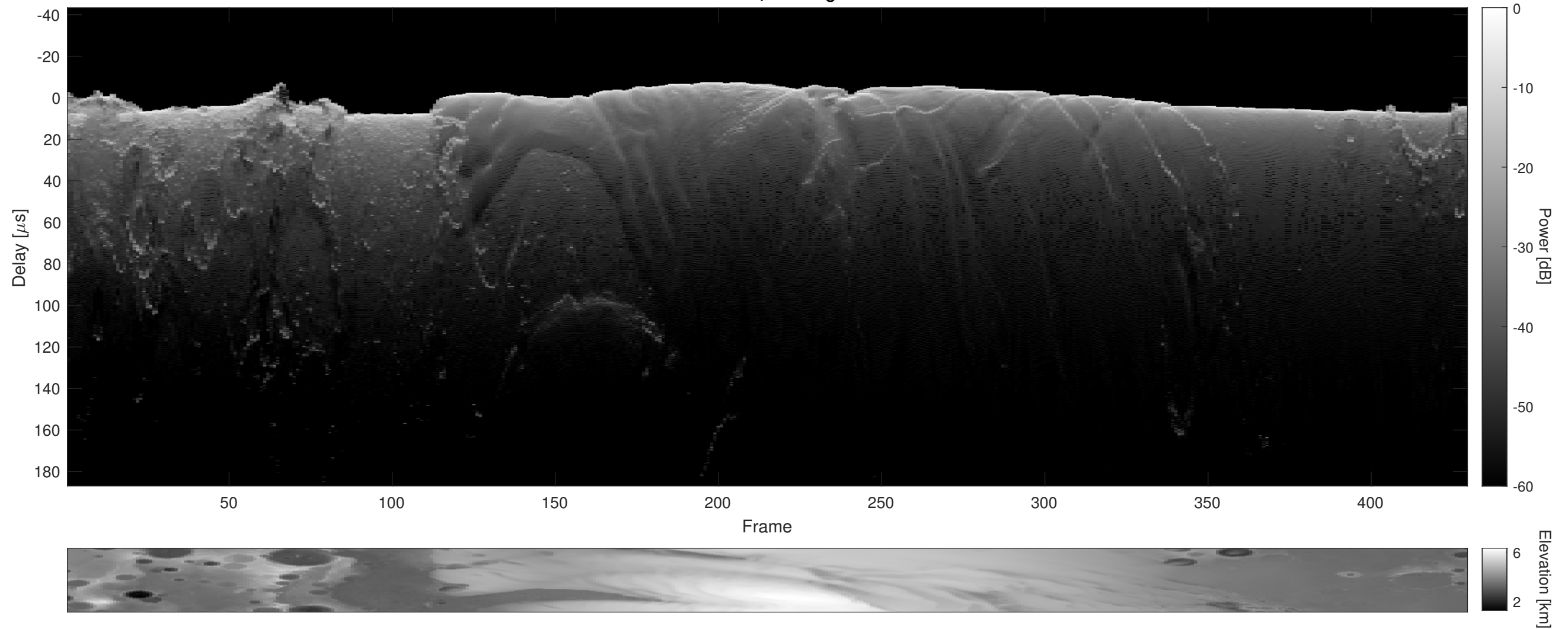
Orbit 19023, Cluttergram
