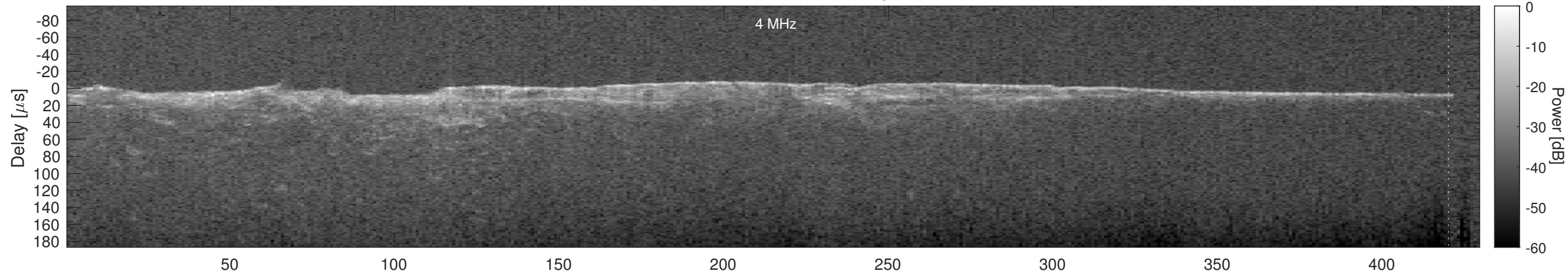
Orbit 19023, Cluttergram
