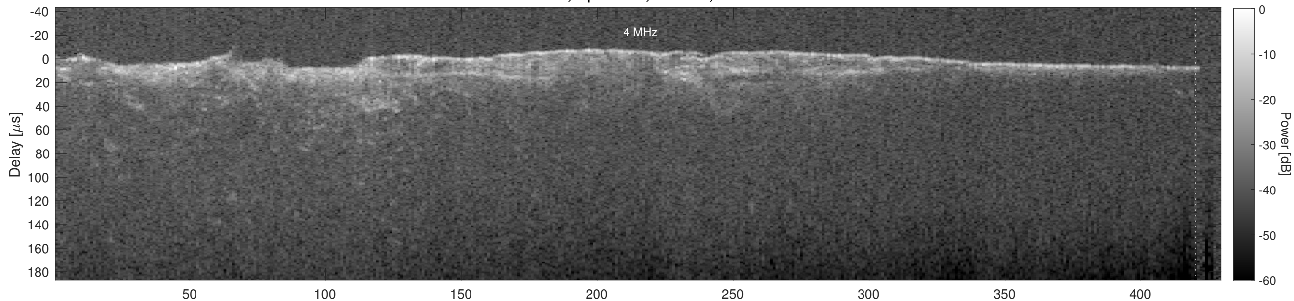
Orbit 19023, Cluttergram
