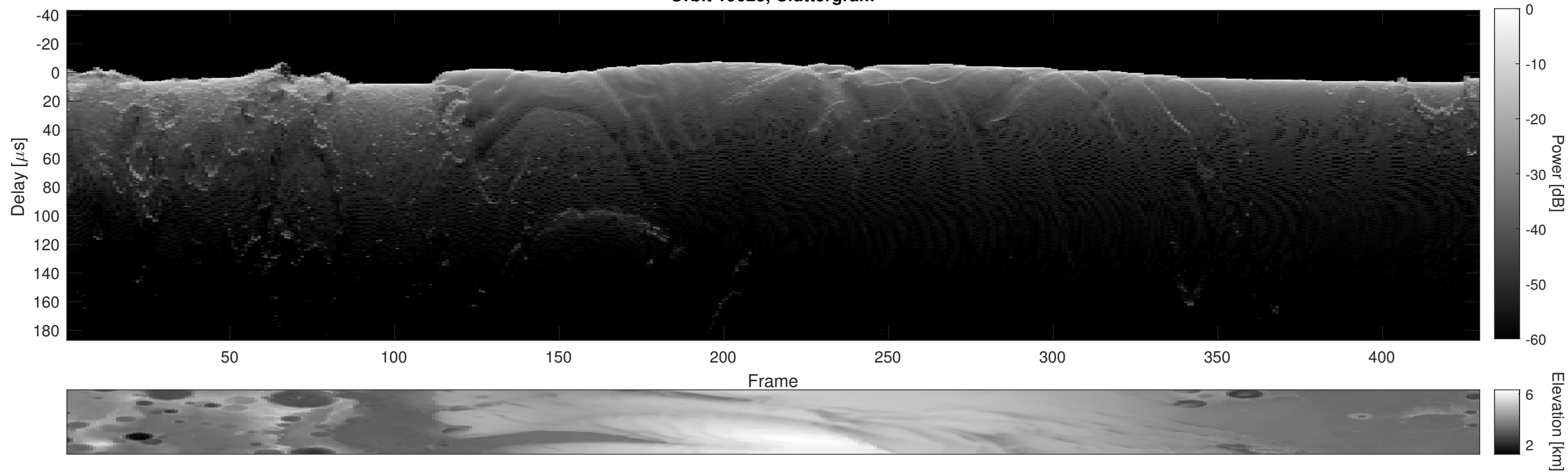
Orbit 19023, Cluttergram
