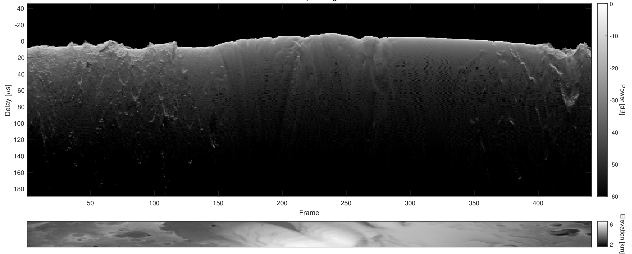
Orbit 19027, Cluttergram
