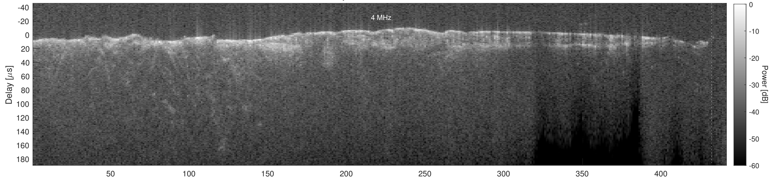
Orbit 19027, Cluttergram
