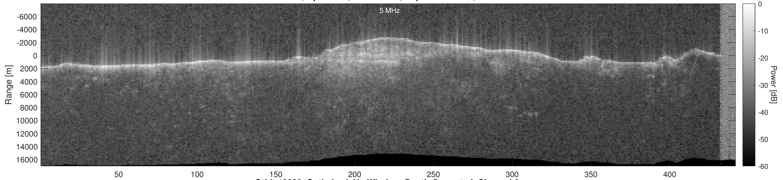
Orbit 19028, Optimized, No Window, Depth-Corrected, Channel 2
