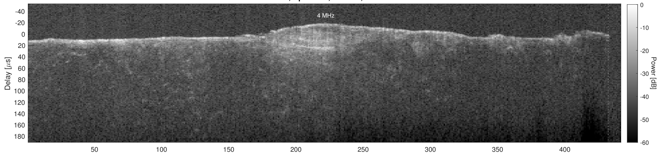
Orbit 19028, Cluttergram
