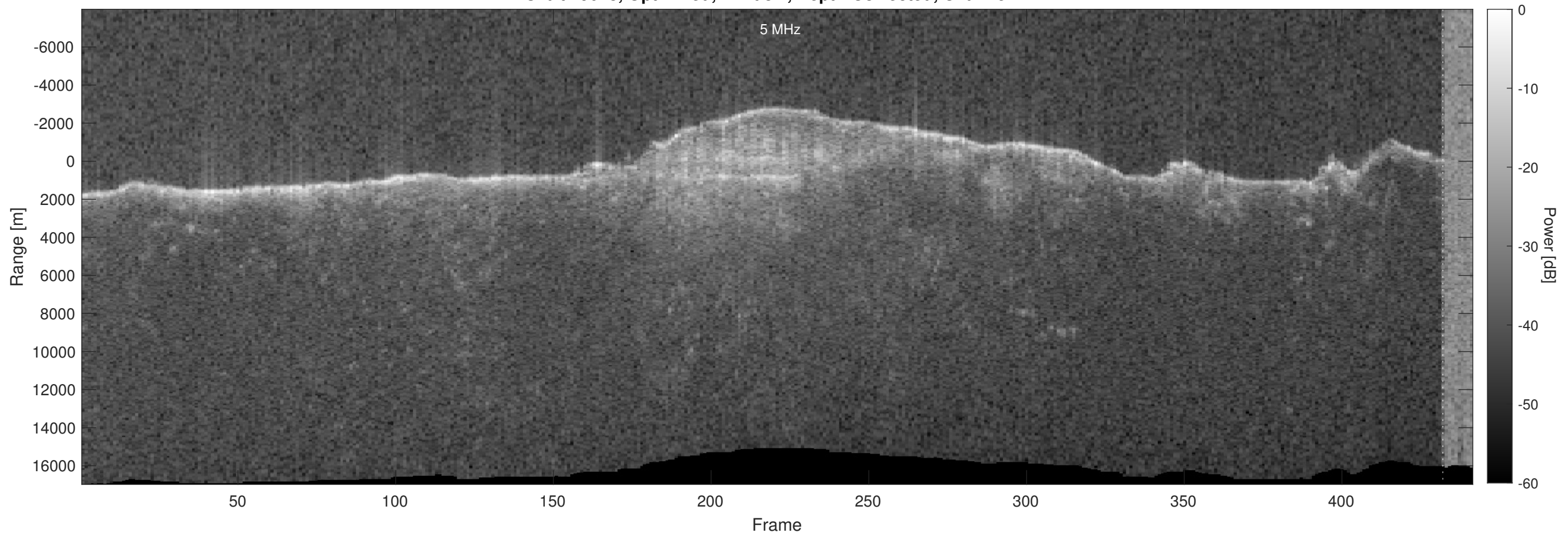
Orbit 19028, Optimized, Window, Depth-Corrected, Channel 2
